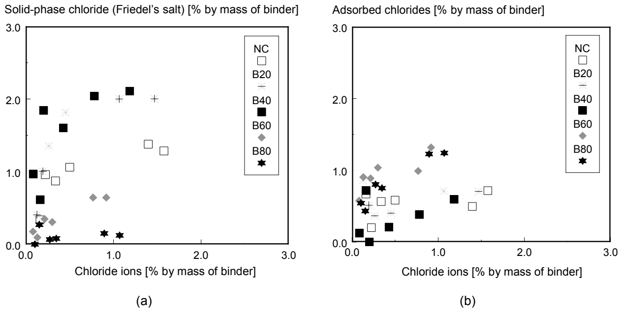
Figure 16 Relationships between quantities of chloride ions and solid-phase and adsorbed chlorides (effects of replacement of cement with ground granulated blast furnace slag)
