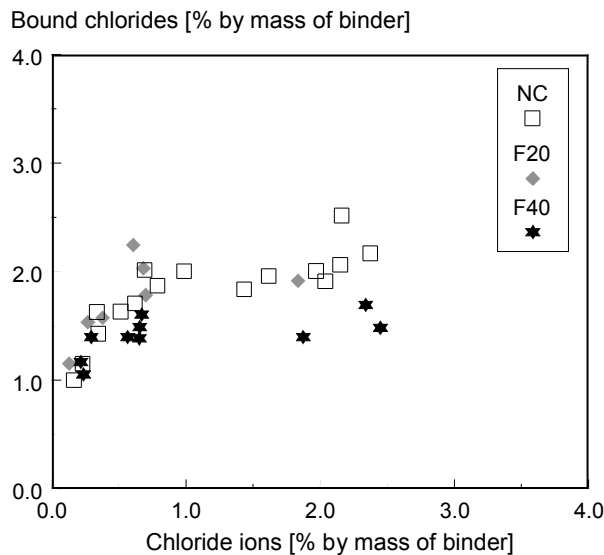
Figure 18 Chloride binding capacity of mortar using fly ash
