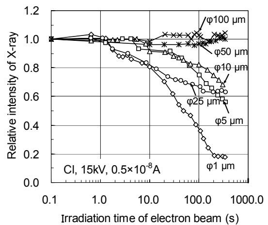
Fig. 12 Count rate change by electron beam irradiation.
