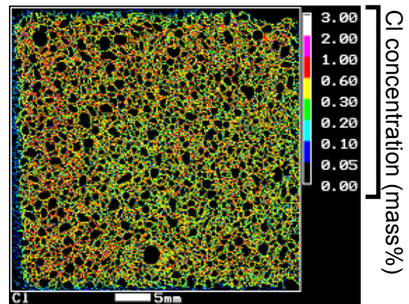
Fig. 13 Area analysis of Cl in mortar by EPMA ( \text{W/C} = 0.50 , \text{S/C} = 3.0 , \text{Cl} = 1.0\ \text{mass}\% -cement).
