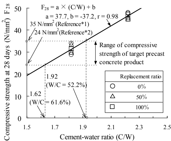
Reference*1: JIS A 5372 Annex 3, RC box culvert 35 N/mm 2 or more Reference*2: JIS A 5371 Annex 2, Boundary block 24 N/mm 2 or more
