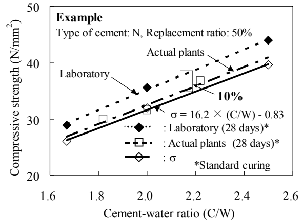
Fig. 9 Example of formula for calculating water-cement ratio.
