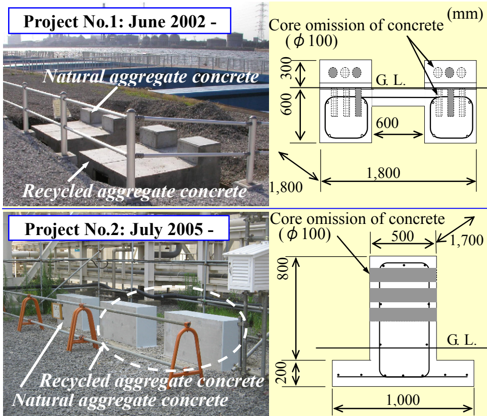
Fig. 12 Outline of samples for monitoring.
