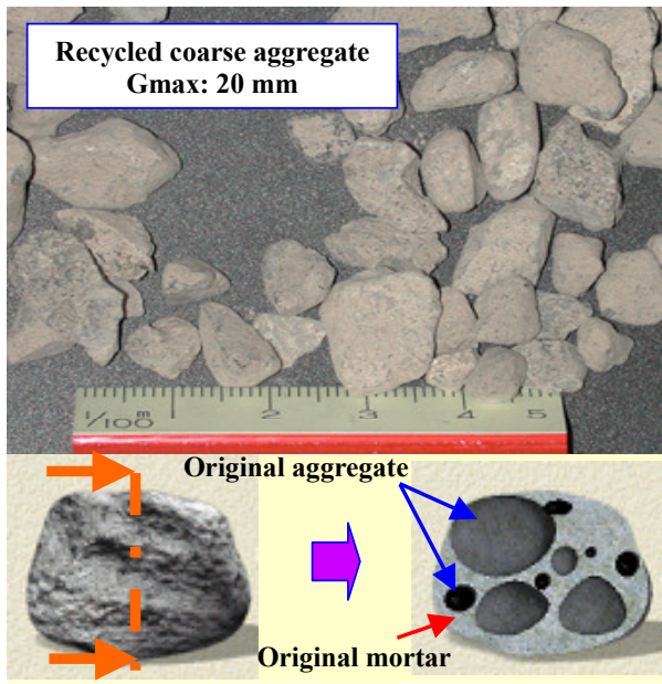
Fig. 4 Appearance of recycled aggregate.
