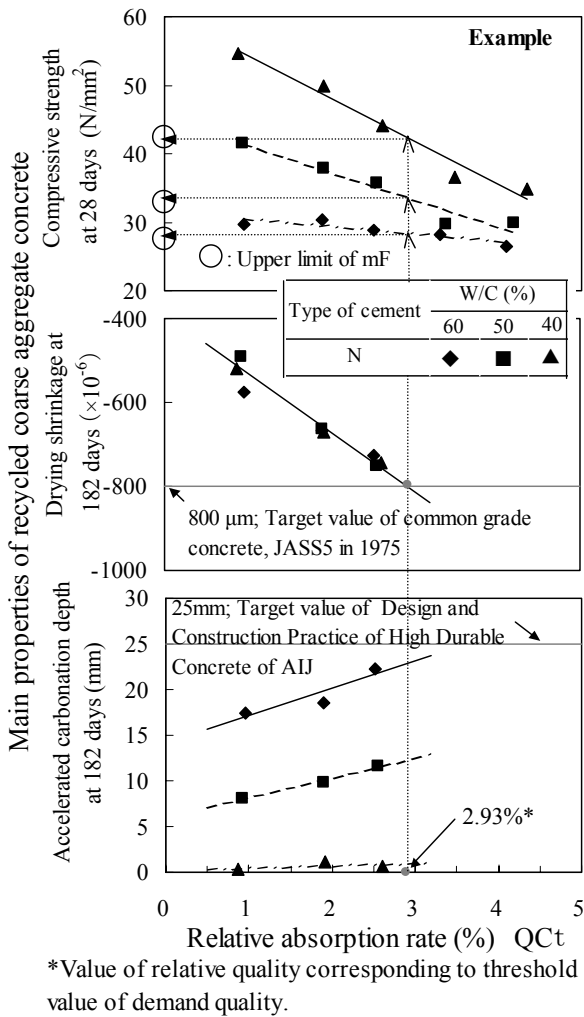
Fig. 8 Example of relationship between relative absorption rate and main properties of recycled coarse aggregate concrete.
