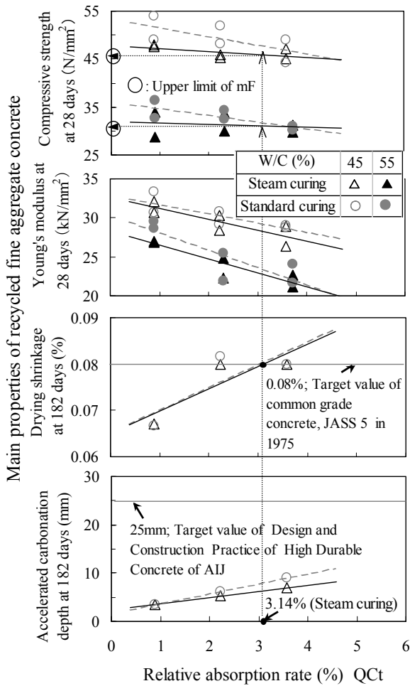
Fig. 15 Relationship between relative absorption rate and main properties of recycled fine aggregate concrete.
