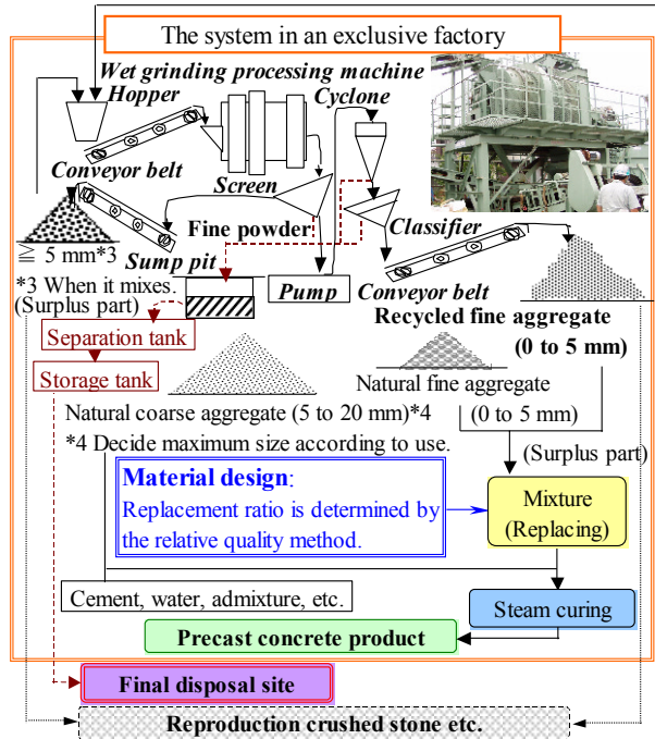
Fig. 5 Developed recycling system for concrete waste.
