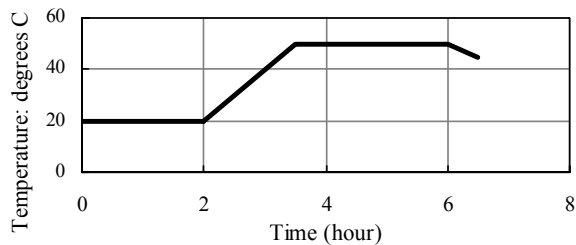
Fig. 14 Cycle of steam curing.
