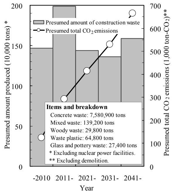
Fig. 1 Presumed amount of construction waste and CO 2 emissions (Buildings owned by TEPCO).
