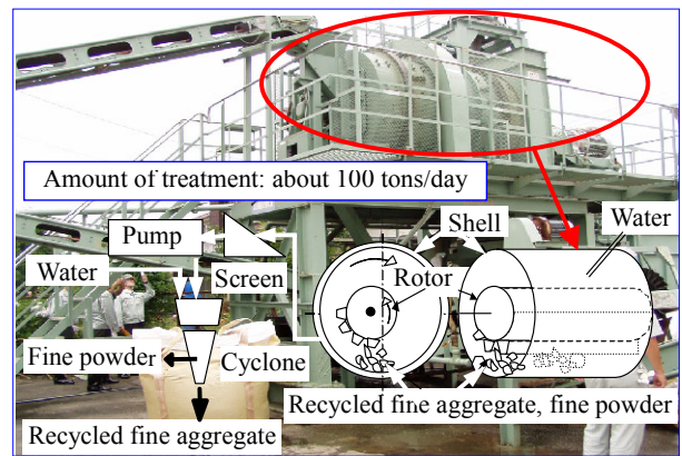
Fig. 13 Outline of wet grinding method.
