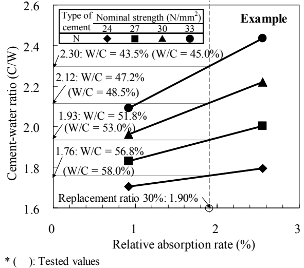
Fig. 10 Example of presumed water-cement ratio on arbitrary replacement ratios
