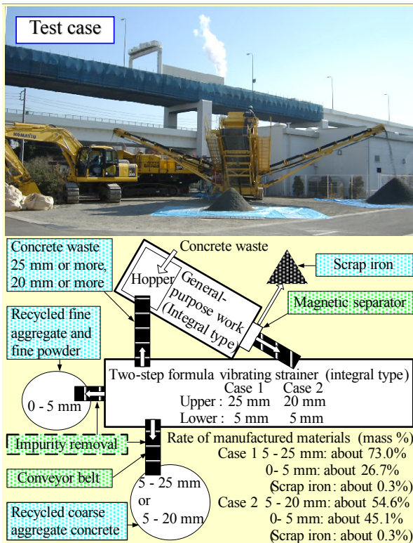
Fig. 6 Manufacturing situation of actual recycled aggregate.
