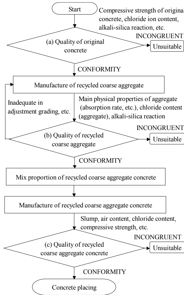
Fig. 11 Quality control flow for recycled coarse aggregate concrete.
